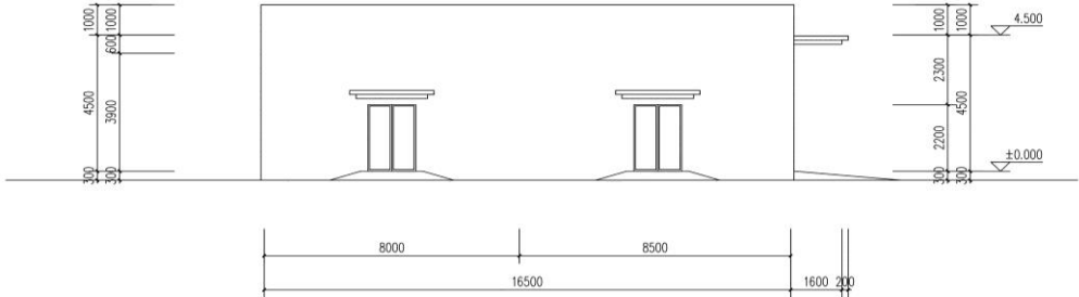
北立面图 1:100 North elevation view
