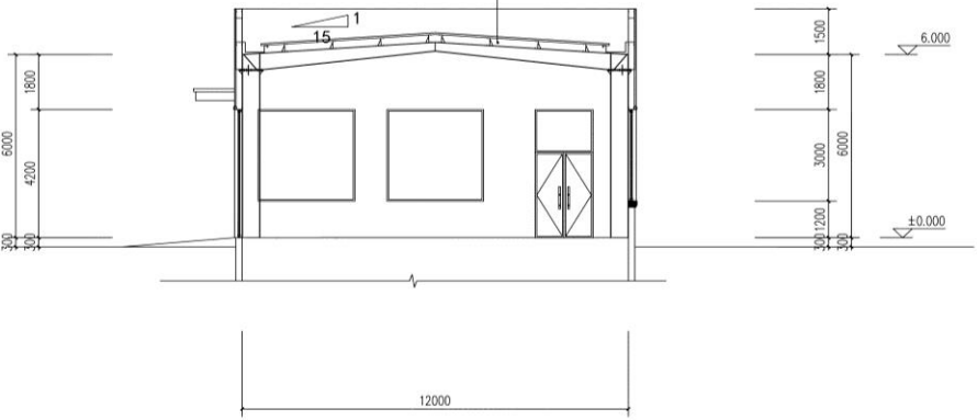
1-1剖面图 1:100 1-1 sectional view
