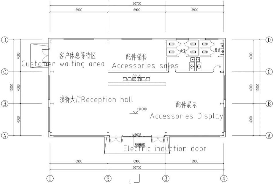
一层平面图 Floor plan of the first floor 1:100
