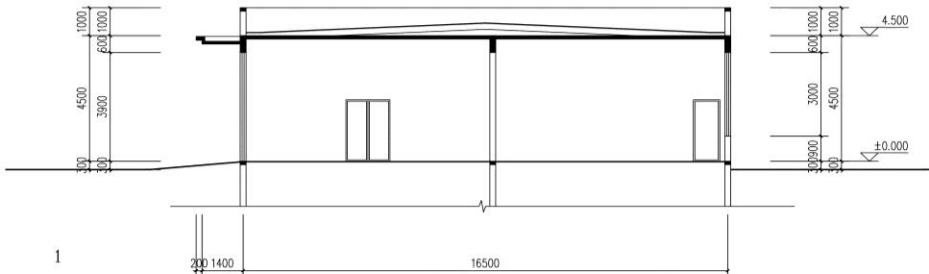
1-1剖面图 1:100 1-1 sectional view
